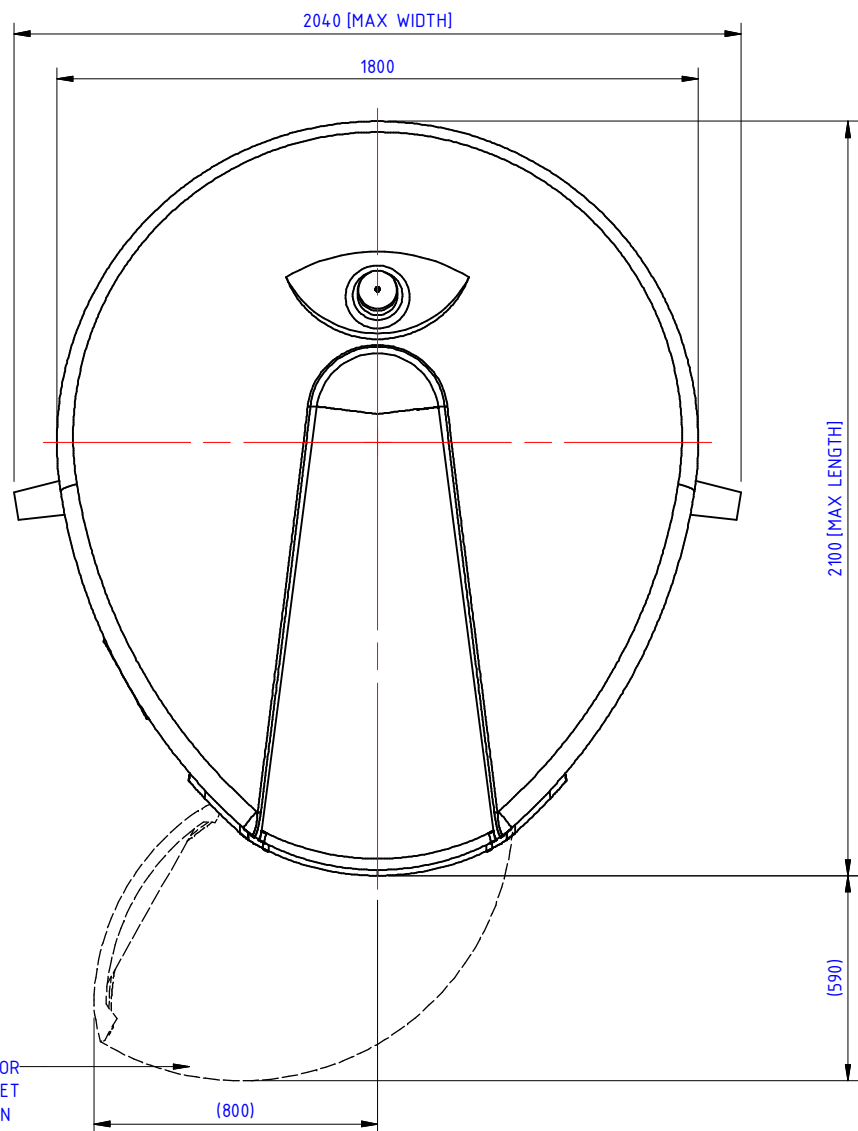
PLAN
