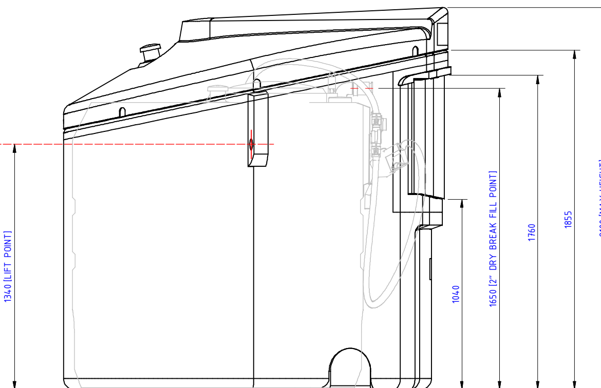
SIDE ELEVATION
