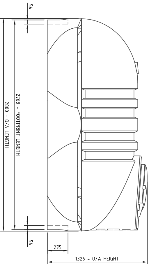
SIDE ELEVATION
