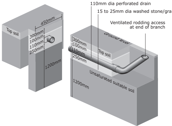
Figure 9 Section through a subsurface percolation trench
