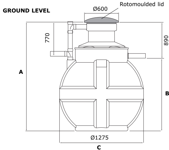
Figure 2 Tank selection
