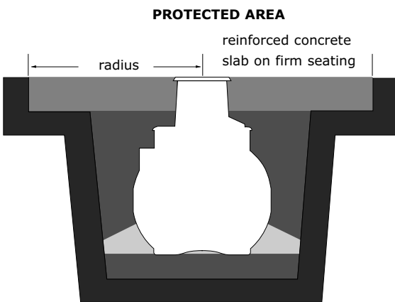
Figure 3 Superimposed loads and protected areas
